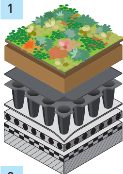
ND 5+1 Drainagesysteem
