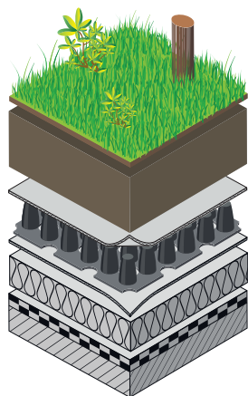
Composition Nophadrain Intensive Green Roof System
