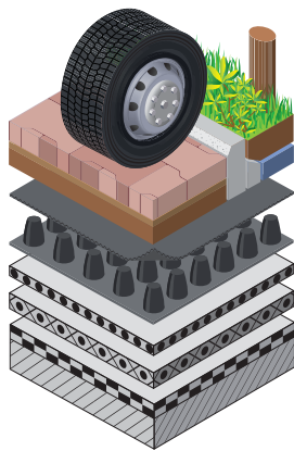
Composition Nophadrain Parking Deck System - HGV
