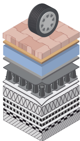
Composition Nophadrain Parking Deck System - cars inverted roof construction
