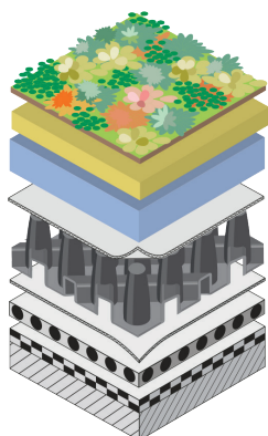
Composition Nophadrain Water Buffering Roof System with ND 6+1v
