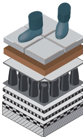
Composition Nophadrain Podium Deck System
