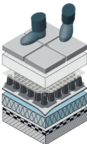
Composition with ND Trasdrain 200sv Drainage System
